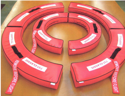
Boeing 737, Bypass & Exhaust Plugs, Folding Donut Ring Type, 300-500 Models
