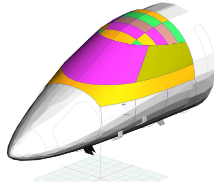
Pilatus PC-24 Cockpit Cover (3D model)
