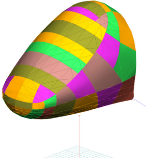
RAF 2000 Gyrocopter Canopy/Nose Cover, 3D model
