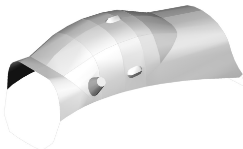
Scheibe SF25 Canopy Cover, 3D model
