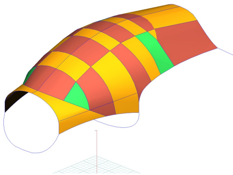
Vivat L-13 Motorglider Canopy Cover, 3D Model
